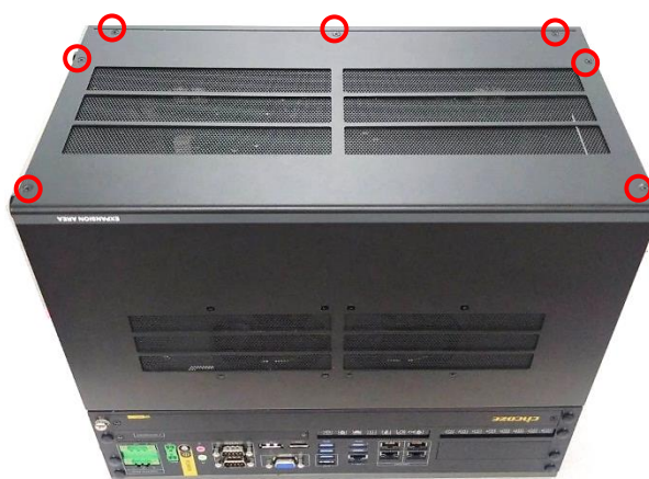
Front Panel
