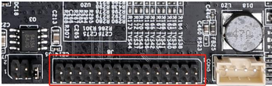
Picture above shows jumper cap positions, from right to left is 3V/5V/12V.
